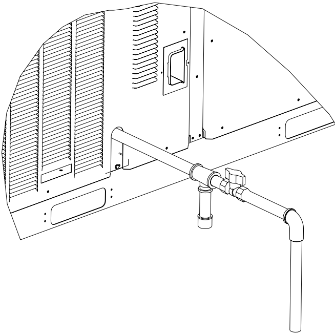
Figure 18: Side Entry Gas Piping
