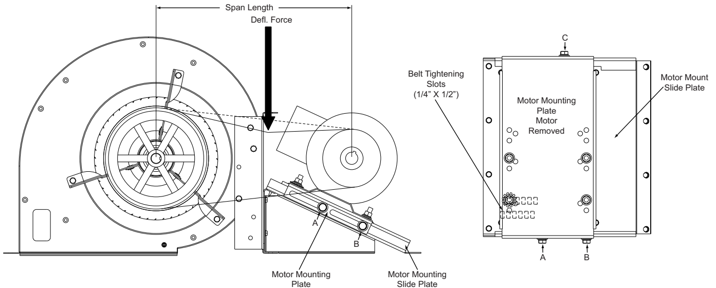
Figure 21: Belt Adjustment
