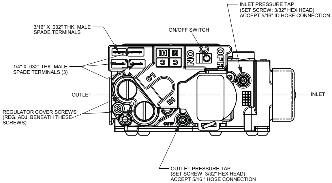
Figure 28: 3 Thru 6 Ton, 1/2" Two Stage Gas Valve
