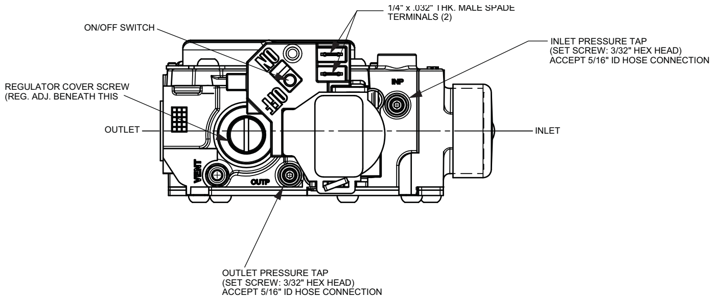
Figure 27: 3 Thru 6 Ton, 1/2" Single Stage Gas Valve
