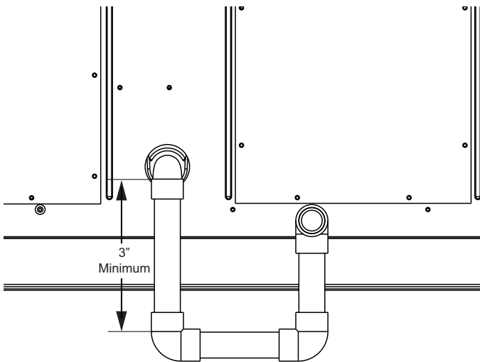
Figure 17: Condensate Drain
