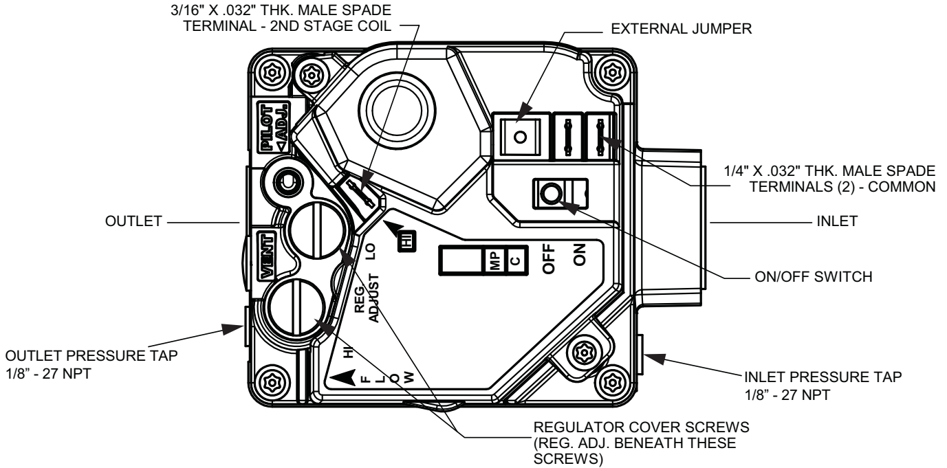
Figure 29: 7.5 Thru 12.5 Ton 3/4” Two Stage Gas Valve
