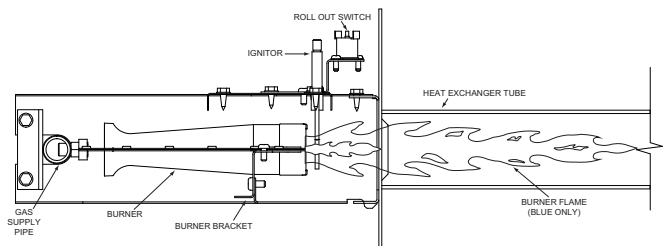
Figure 26: Typical Flame
